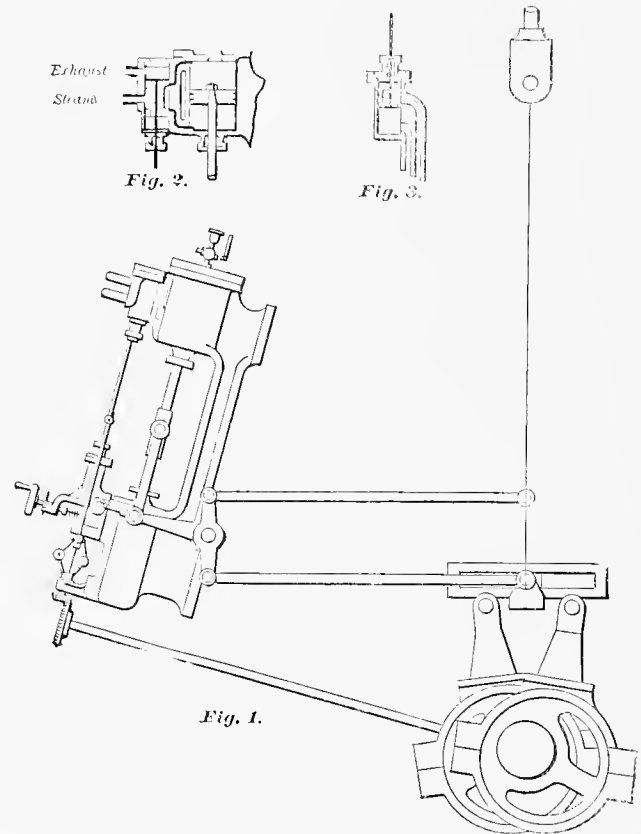
CHASE'S VALVE GEAR AND MARINE GOVERNOR.
